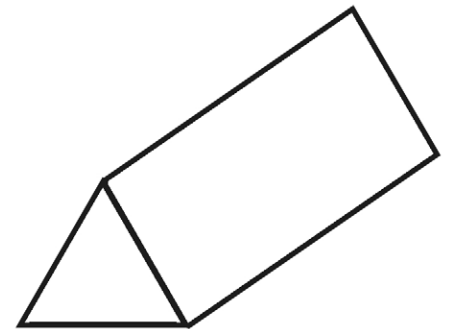
triangular prism
